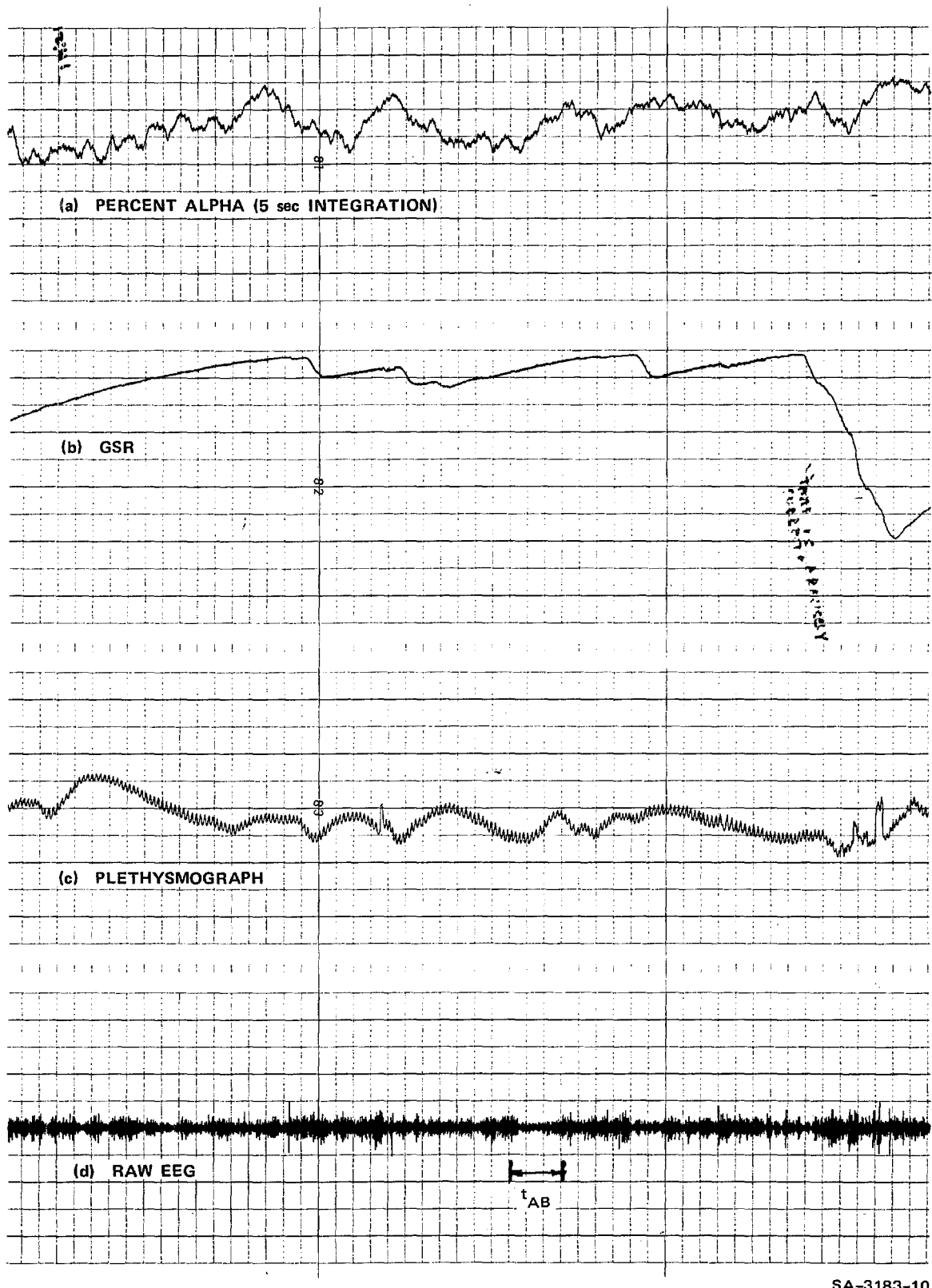
FIGURE 24 POLYGRAPH DATA
